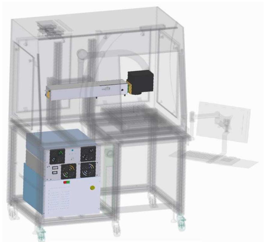
laser unit AQUILA 120 (straight beam delivery)
